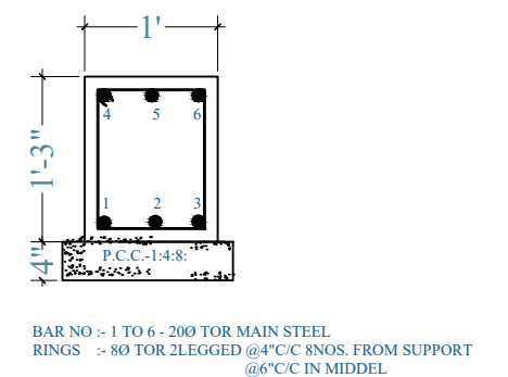
BEAM 'PB5'
