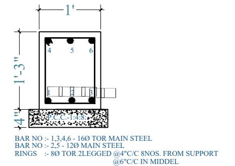
BEAM 'PB2'
