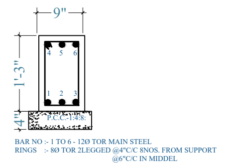
BEAM 'PB3'
