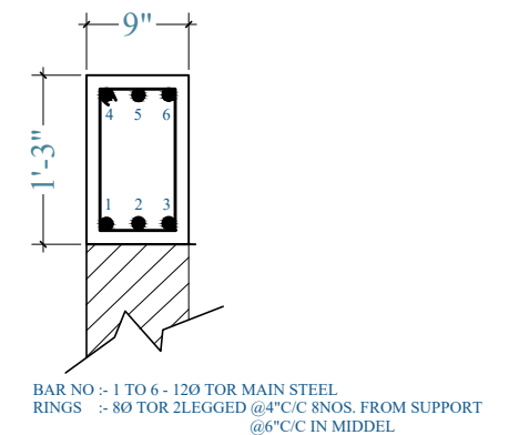
BEAM 'PB4'
